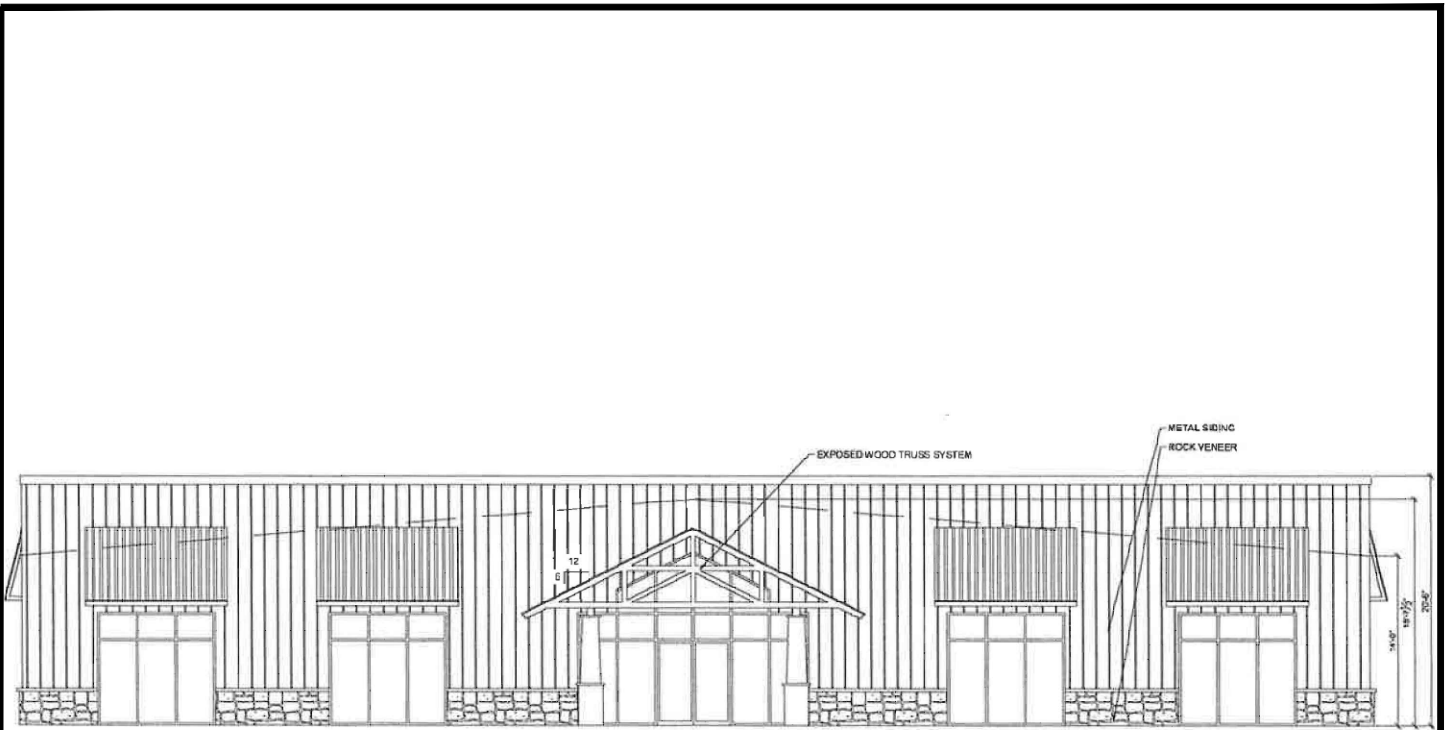
CLIMATE STORAGE SOUTH ELEVATION ————— SCALE: 1/4" = 1'-0"
