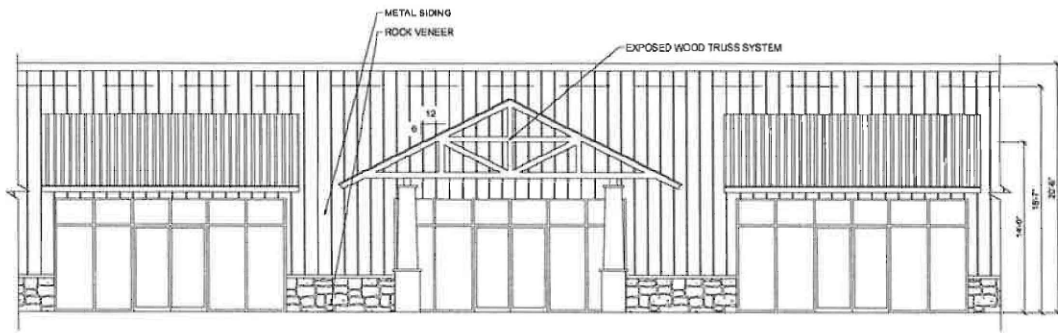
OFFICE / RETAIL PARTIAL SOUTH ELEVATION ————— SCALE: 1/4" = 1'-0"
